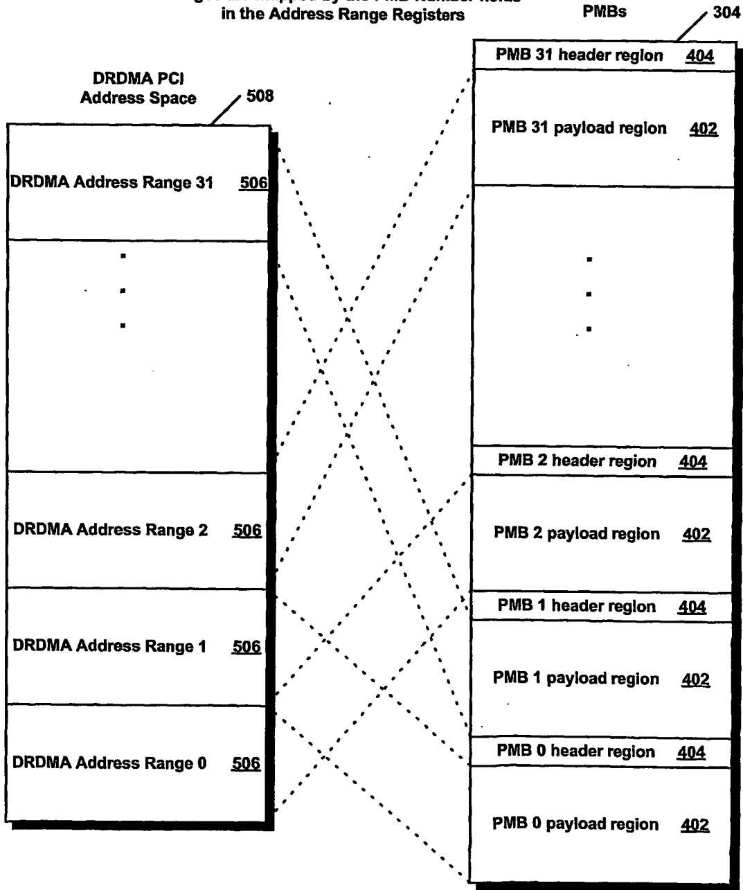
DRDMA Address Range to PMB Payload Region Mapping
